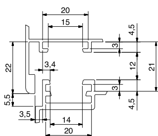
EUROGROOVE PROFILE CAMARA EUROPEIA
